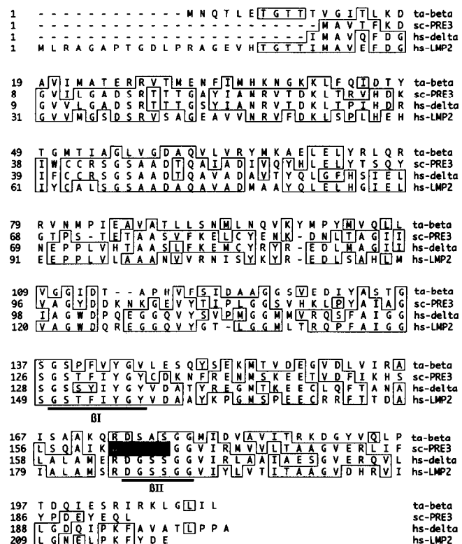
Fig. 3. Alignment of the \beta -subunit from archaeobacteria T. acidophilum [38], the yeast Pre3 protein, the Hs \delta subunit of the human proteasome [28], and the human MHC-encoded Lmp2 (Ring12) protein [12]. Gaps are inserted for optimal alignment. Identical amino acids are indicated by boxes. The glutamine synthetase motif is shown by the filled box. The consensus PROS box domains defining members of the \beta -type proteasome family are underlined.
